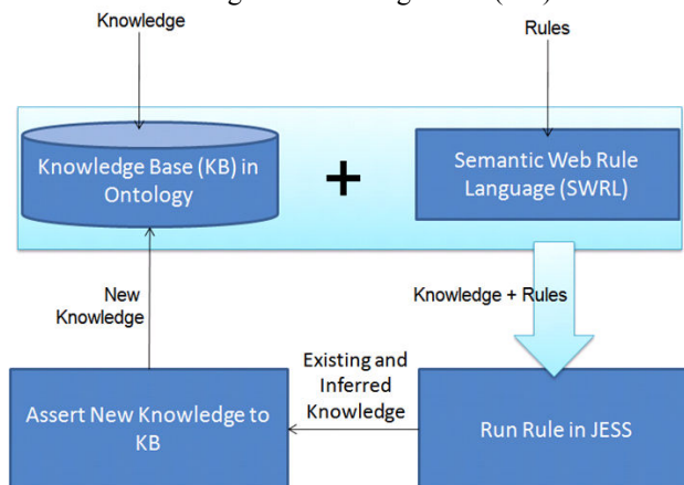
Figure 3. Infer new knowledge process
