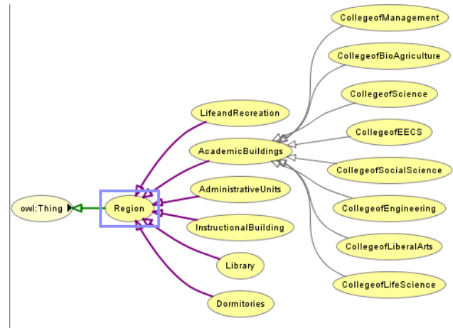
Figure 6. NTU location ontology class hierarchy
